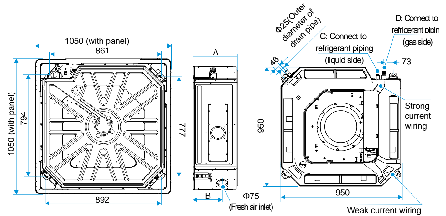
Figure 2.1: 16.0-18.0kW Four-way Cassette dimensions (unit: mm)
