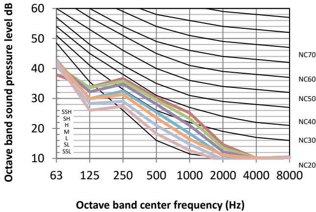
Figure 8.4: MIH45Q4HN18 octave band levels
