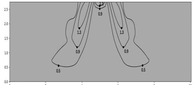
Figure 9.20: MIH180Q4HN18 heating at 300s
