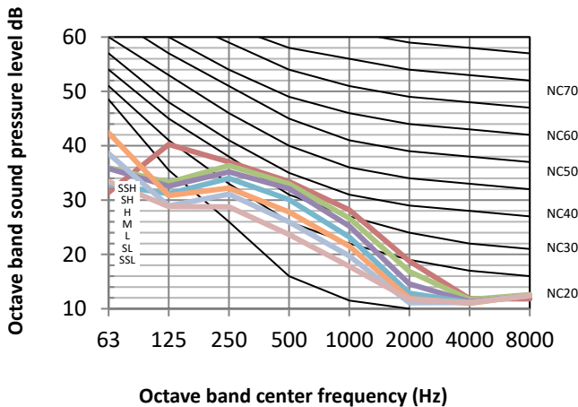
Figure 8.4: MIH45Q4HN18 octave band levels
